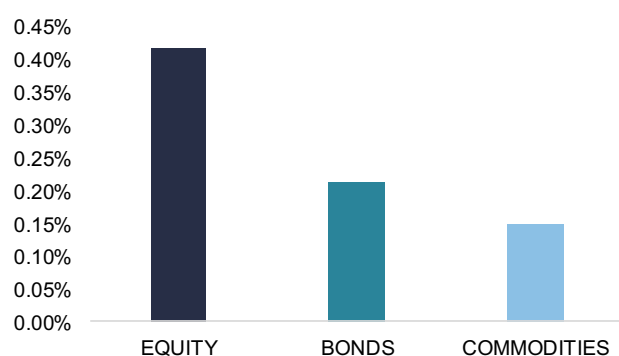
Individual VaR
